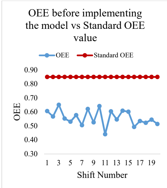
Figure 6. OEE before implementing the model vs Standard OEE.
