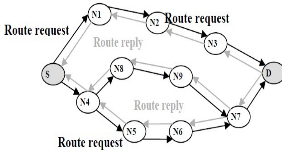
Figure 3: Reactive Routing Protocol [9]
