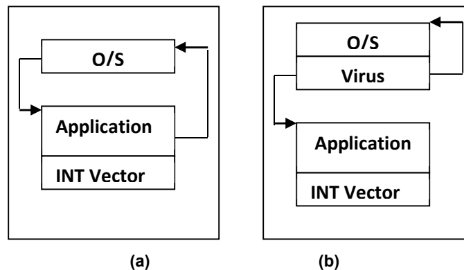
Figure 3: Interrupt routing before and after infection
