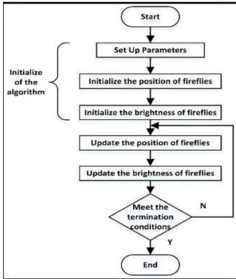
Fig. 1. Procedure Block for Firefly Algorithm (Source Aiming Liu, et al. 2017)
