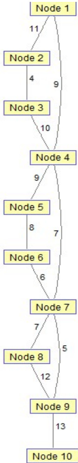
Fig. 2.0 OSPF + FIREFLY
