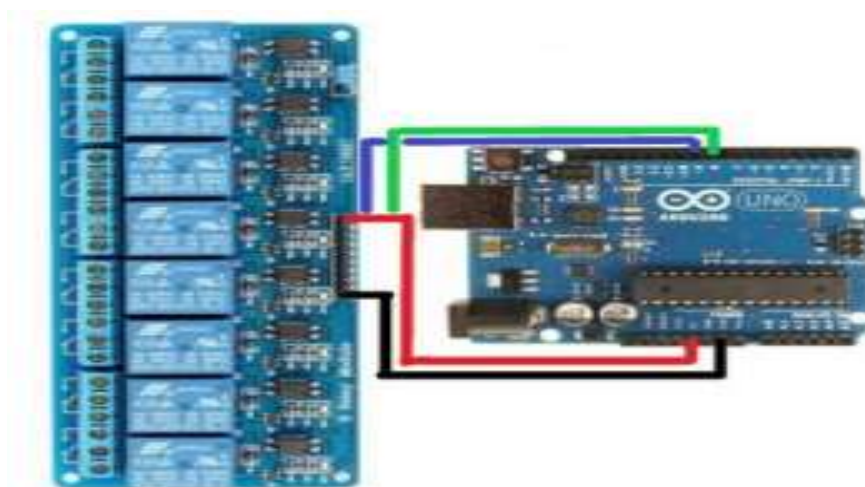
Figure 7. Relay Module
